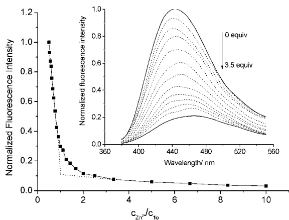
Figure 2. Fluorescence intensity changes at 440 nm with different molar ratio of \text{Zn}^{2+} and 1o in THF/ water solution (100:1, v/v) ( 1o from 2 \times 10^{-5} to 1 \times 10^{-6} M, \text{Zn}^{2+} with the fixed concentration of 1 \times 10^{-5} M). (Inset) Fluorescence spectral changes of 1o ( 1 \times 10^{-5} M) by the addition of \text{Zn}^{2+} from 0 to 3.5 equiv.
