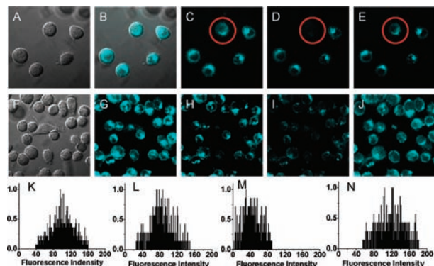
Figure 3. CLSM images of KB cells incubated with 1o for 20 min at 25 °C ( 1 \times 10^{-5} \text{ M} in PBS/ DMSO, 100:2, v/v). (A, F) Bright-field transmission image of KB cells. (B) Overlay image of A and C. Confocal fluorescence image of (C) original state, (D) irradiated by 405 nm light (2 mW, 3 min) for one selected cell and (E) recovered by 633 nm light (0.7 mW, 40 min). Confocal fluorescence image of (G) original state of F, and incubation by \text{Zn}^{2+} solution with the concentrations of (H) 5 \times 10^{-5} \text{ M} , (I) 1 \times 10^{-4} \text{ M} . (J) Recovered by 5 \times 10^{-4} \text{ M} EDTA solution. (K), (L), (M), (N) were the distribution of fluorescence intensity of (G), (H), (I), (J), respectively.
