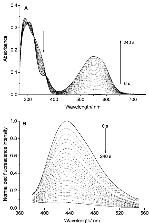
Figure 1. (A) Absorption and (B) fluorescence emission changes of 1o in THF ( 1 \times 10^{-5} M) upon irradiation with 365 nm light ( \lambda_{\text{ex}} = 330 nm).
