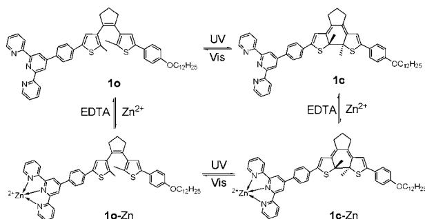
Scheme 1. Chemical Structure Changes of Compound 1o
